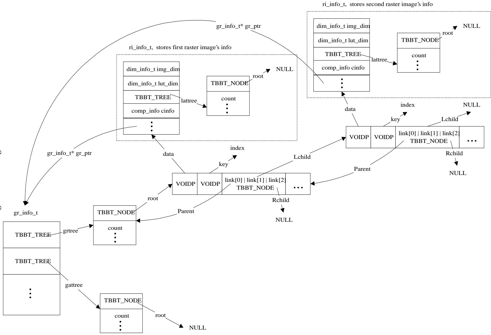
Data structures storing two raster images
