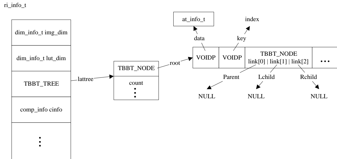
FIGURE 8r Illustration of data structure ri_info_t
