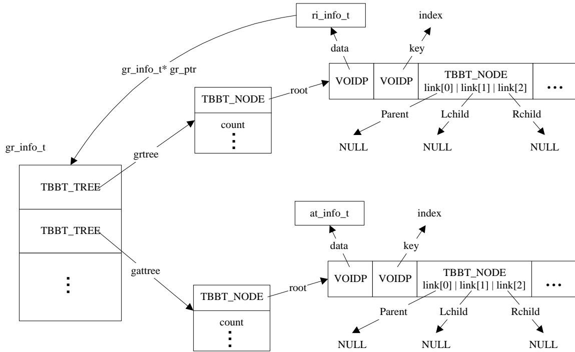
FIGURE 8q Illustration of data structure gr_info_t
